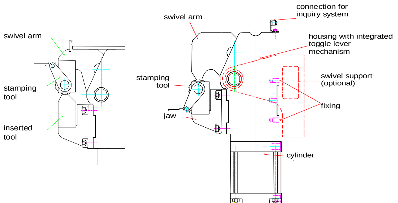
Fig. 1: Basic construction of the marking unit
